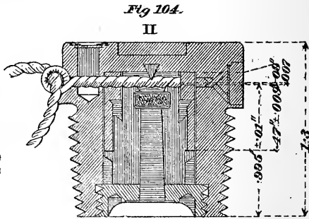
Royal laouratory percussion fuzes I and II.
